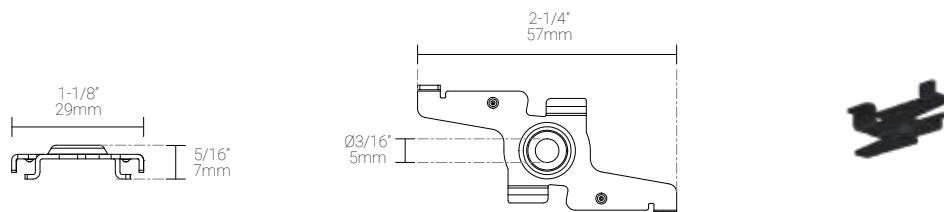
Ceiling Clamp
